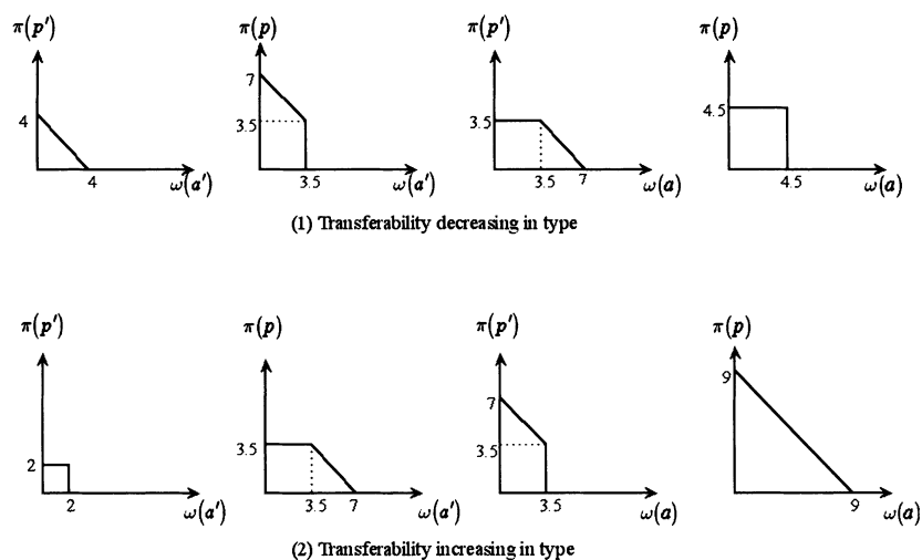
FIGURE 2.1.—Utility possibility frontiers.
