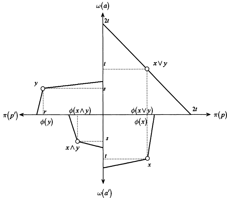
FIGURE A.1.—GID holds but QSM is violated.
