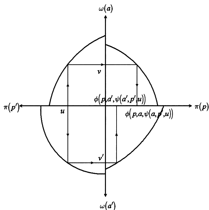
FIGURE 4.1.—Generalized increasing differences.
